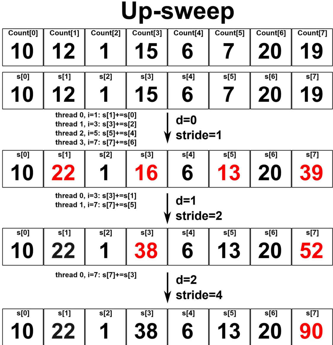
Figure 8: Blelloch scan up-sweep array visualization.
